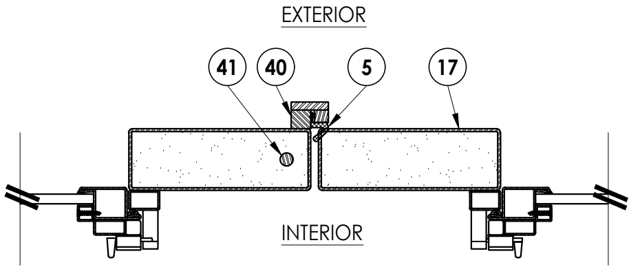
2 3 HORIZONTAL CROSS SECTION Inswing Shown (Outswing Similar)
