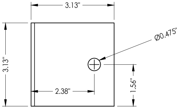
32 ANCHORING ANGLE
