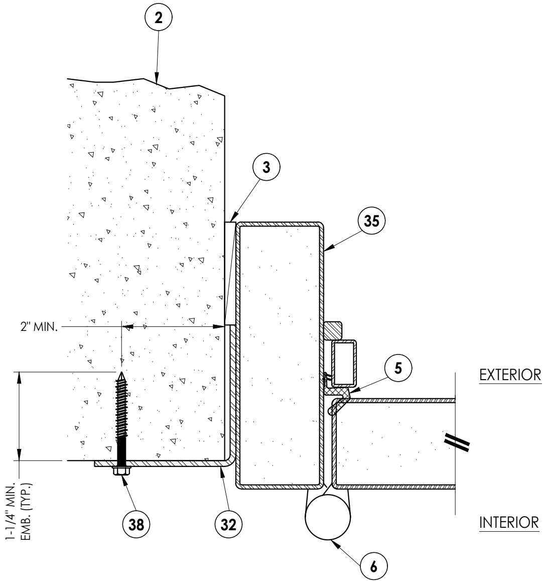
1 HORIZONTAL CROSS SECTION 4 Direct To Masonry Inswing Shown (Outswing Similar)
