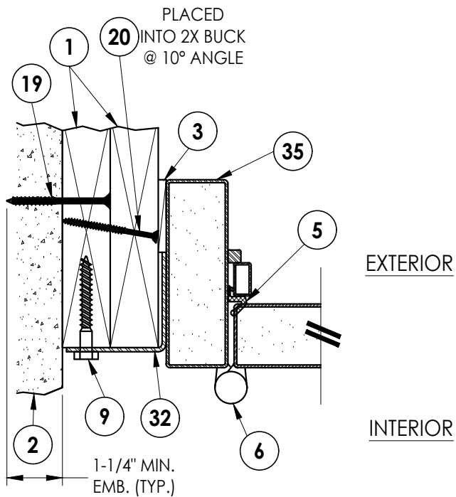
1 3 HORIZONTAL CROSS SECTION Inswing Shown (Outswing Similar)
