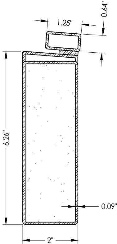
18 BOTTOM RAIL Foam filled
