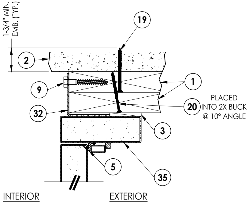
3 3 VERTICAL CROSS SECTION Inswing Shown (Outswing Similar)
