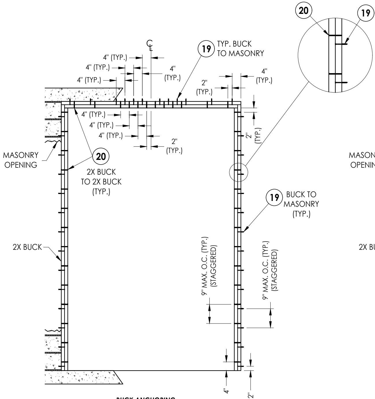
BUCK ANCHORING (Max. design pressure \pm 100 psf)
