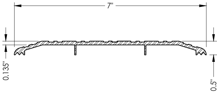
30 ADA THRESHOLD
