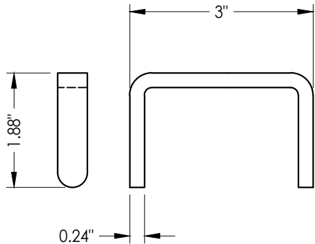
34 LATCH KEEPER
