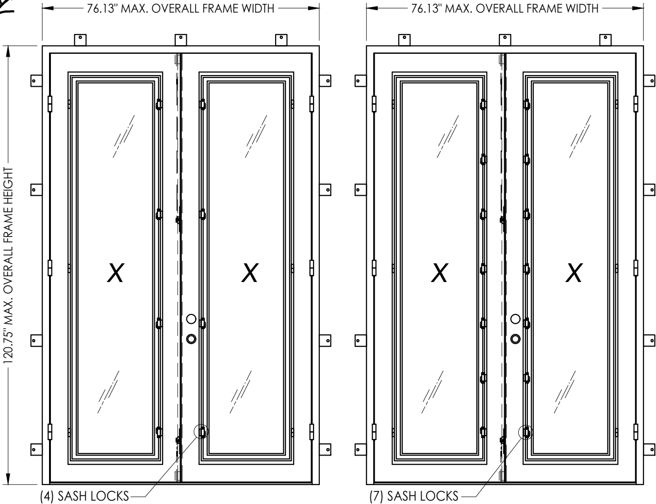
GLAZED DOOR WITH 4 SASH LOCKS
