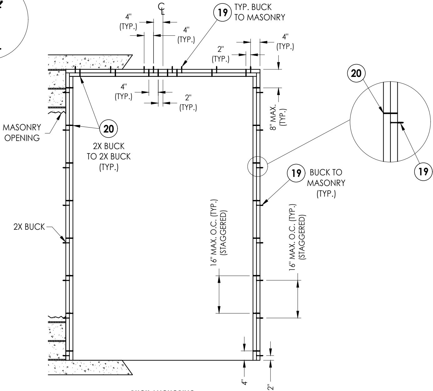
BUCK ANCHORING (Max. design pressure \pm 65 psf)
