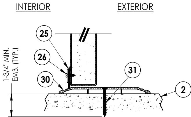
4 3 VERTICAL CROSS SECTION Inswing Shown (Outswing Similar)
